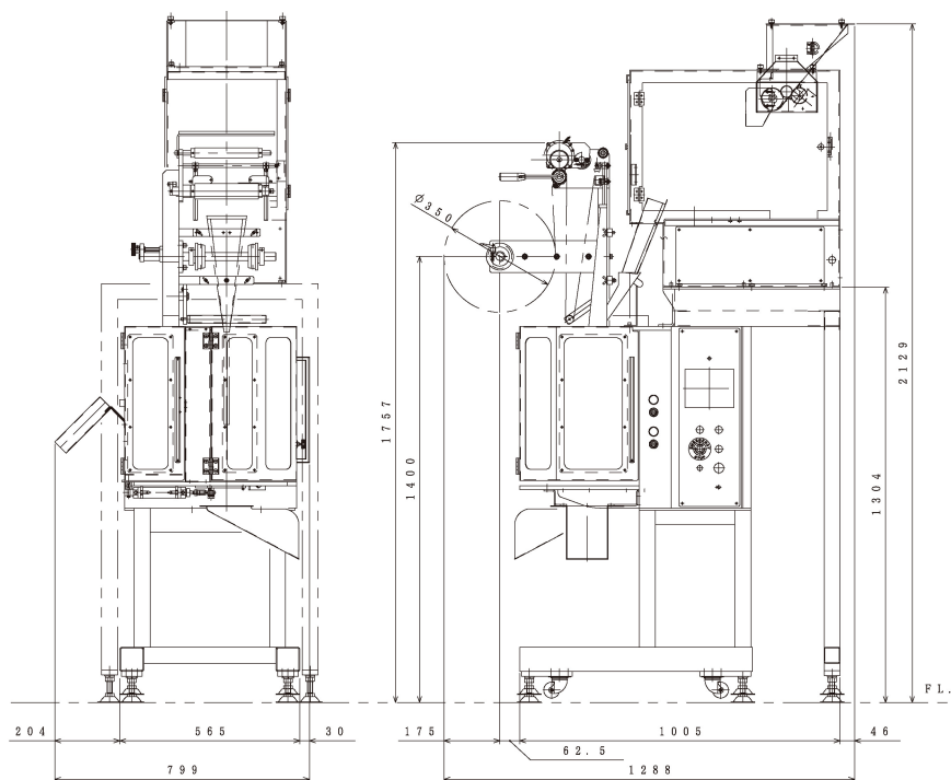
FP-CS+FW-LSA(オプション)
